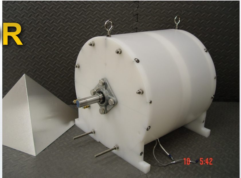
Photo of a 6kw Sp500 AC Generator. Can also output DC if desired. From our Sp500 Model # 4
