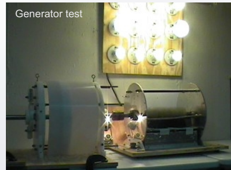
Sp500 Model # 4, lighting 12 light bulbs!
